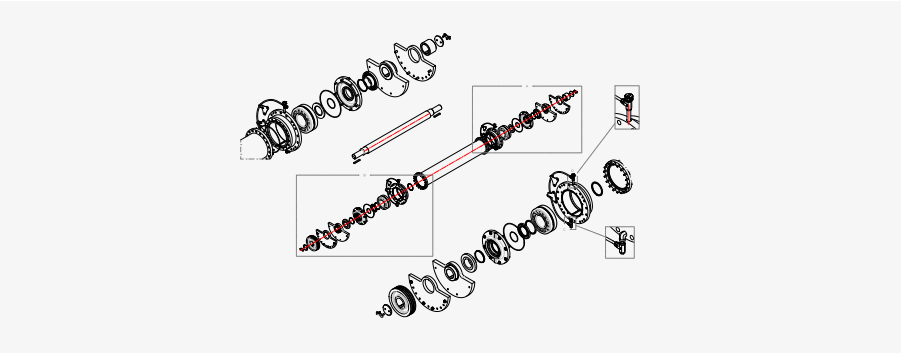
STE exciter – shaft, counterweights, bearings and housings.
